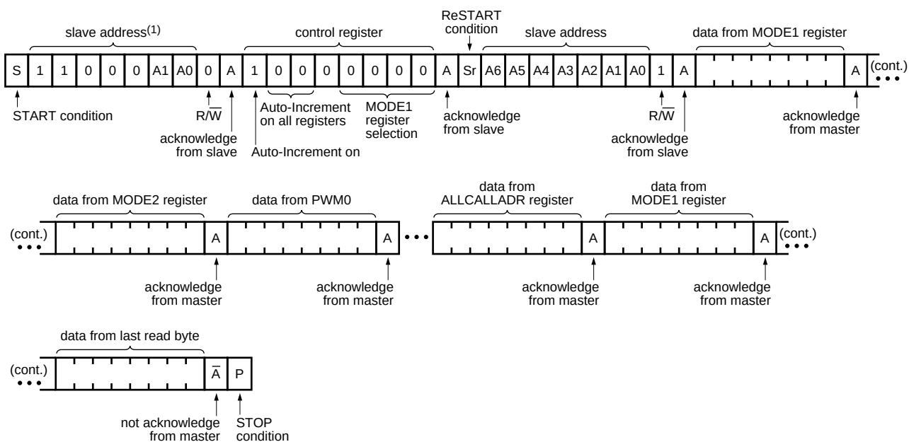
Fig 18. Read all registers using the Auto-Increment feature
