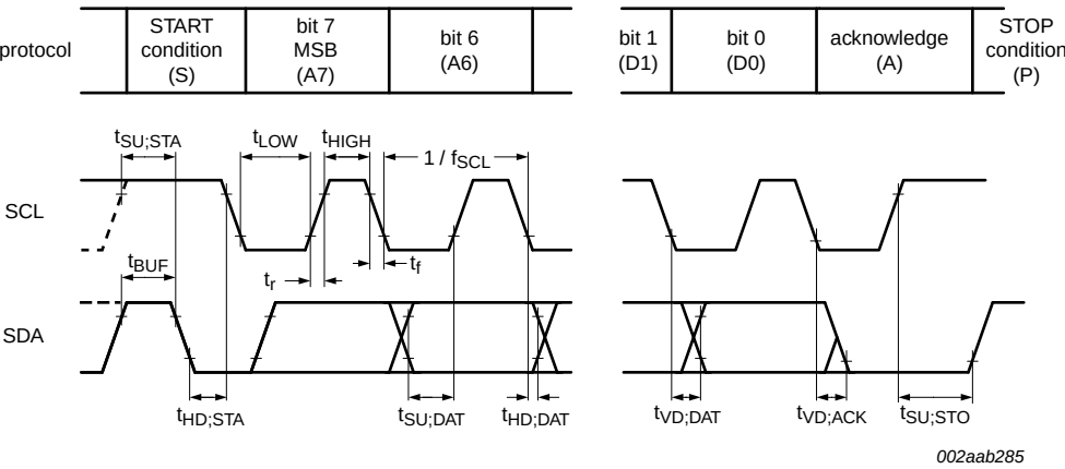
Fig 23. I 2 C-bus timing diagram
