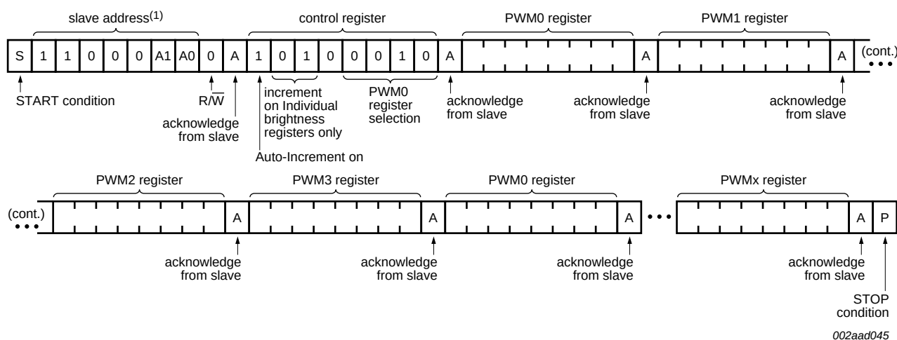
Fig 17. Multiple writes to Individual brightness registers only using the Auto-Increment feature
